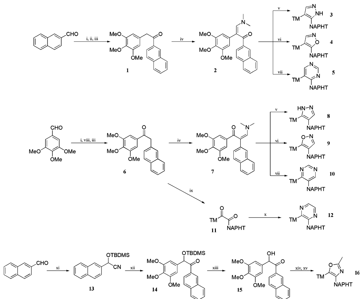
Scheme 1. Reagents and conditions: (i) 1,3-propanedithiol, \text{BF}_3 \cdot \text{Et}_2\text{O} , \text{CHCl}_3 , 0 °C to rt (91%); (ii) BuLi, THF, −78 °C, then 3,4,5-trimethoxybenzyl bromide, THF, −40 °C (93%); (iii) \text{HgO} , \text{BF}_3 \cdot \text{Et}_2\text{O} , THF/ \text{H}_2\text{O} (71%); (iv) dimethylformamide dimethylacetal, toluene, reflux (86%); (v) \text{NH}_2\text{NH}_2 \cdot \text{HCl} , EtOH, 4 Å molecular sieves, reflux (81%); (vi) \text{HONH}_2 \cdot \text{HCl} , \text{Na}_2\text{CO}_3 , AcOH, MeOH/ \text{H}_2\text{O} , reflux (77%); (vii) \text{NH}_4^+ \text{HCOO}^- , \text{HCONH}_2 , \text{HCOOH} , reflux (58%); (viii) BuLi, THF, −78 °C, then 2-bromomethylnaphthalene, THF, −40 °C (97%); (ix) \text{SeO}_2 , toluene, reflux (98%); (x) ethylenediamine, AcOH, reflux (84%); (xi) KCN, \text{CH}_3\text{CN} , \text{ZnI}_2 , TBDMSCl (68%); (xii) LDA, THF, −78 °C, then 3,4,5-trimethoxybenzaldehyde, THF, −78 °C (83%); (xiii) HCl, \text{H}_2\text{O} /THF, (79%); (xiv) \text{Ac}_2\text{O} , DMAP, DCM (96%); (xv) \text{NH}_4^+ \text{AcO}^- , AcOH, reflux (69%). Abbreviations: TM: 3,4,5-trimethoxyphenyl; NAPHT: naphth-2-yl.
