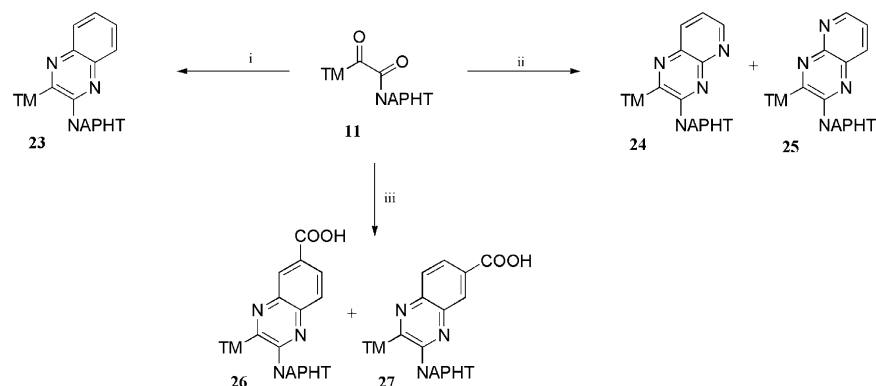
Scheme 3. Reagents and conditions: (i) o -phenylenediamine, AcOH, EtOH, reflux (98%); (ii) 2,3-diaminopyridine, AcOH, reflux (56%); (iii) 3,4-diaminobenzoic acid, AcOH, reflux (67%). Abbreviations: TM: 3,4,5-trimethoxyphenyl; NAPHT: naphth-2-yl.
