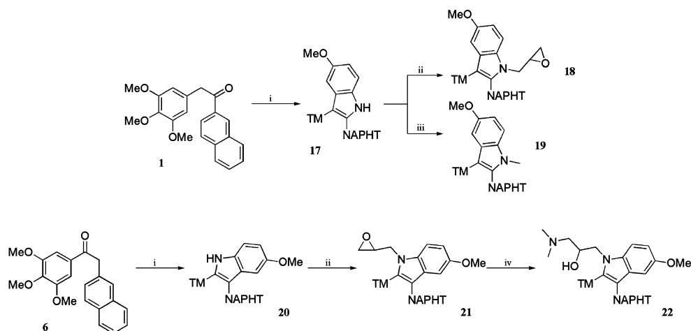
Scheme 2. Reagents and conditions: (i) p -methoxyphenylhydrazine, EtOH, AcOH, reflux (54%); (ii) NaOH, epichlorohydrine, \text{Bu}_4\text{N}^+ \text{HSO}_4^- , benzene (48%); (iii) NaH, MeI, DMF (75%); (iv) N,N -dimethylamine, EtOH (90%). Abbreviations: TM: 3,4,5-trimethoxyphenyl; NAPHT: naphth-2-yl.
