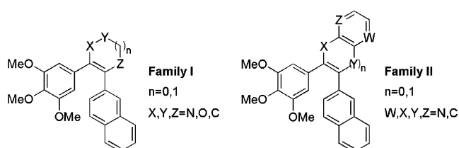
Figure 2. Structure of the designed analogues.
