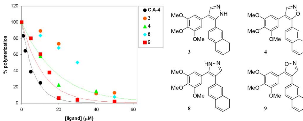
Figure 3. Inhibition of tubulin polymerization (as microtubule protein, MTP), expressed as percentage of polymerization for noninhibited protein. MTP concentration is 1.5 mg/mL.
